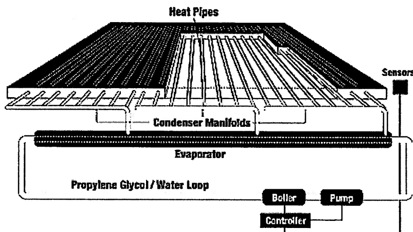
Figure 4. Schematic of the VDOT anti-icing system.
